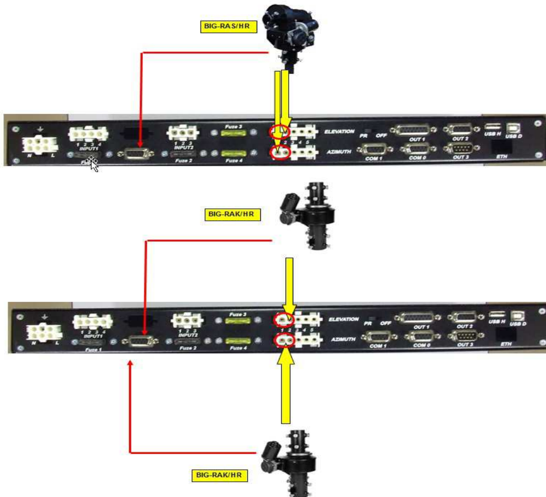
Picture below shows connection of the rotor type /HR:
